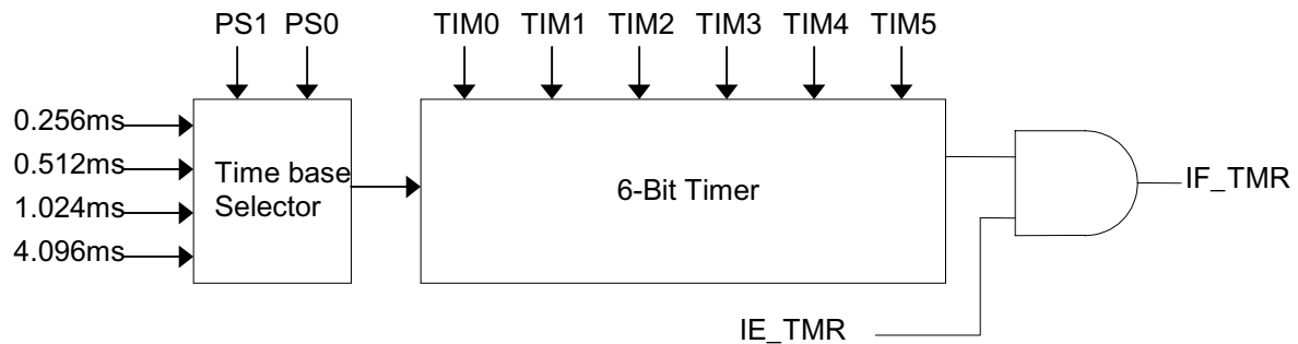
Fig.11 Block diagram of Timer
