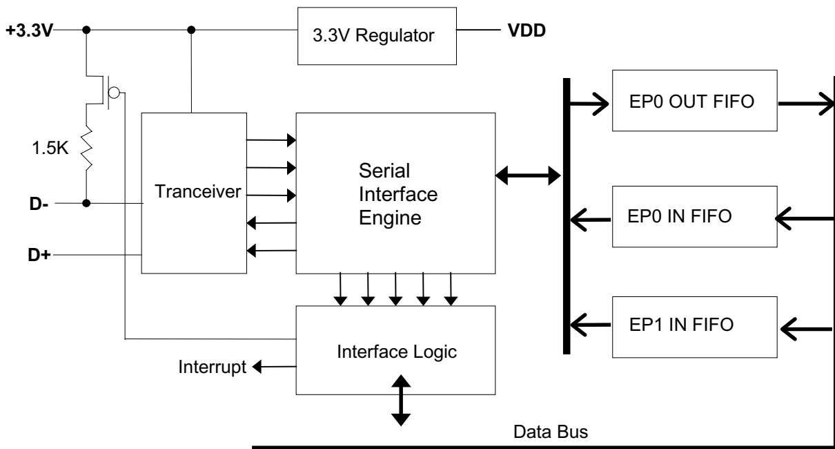
Fig.14 Block diagram of USB function
