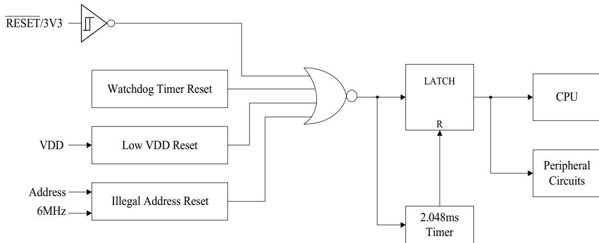
Fig. 1 Reset Signals
