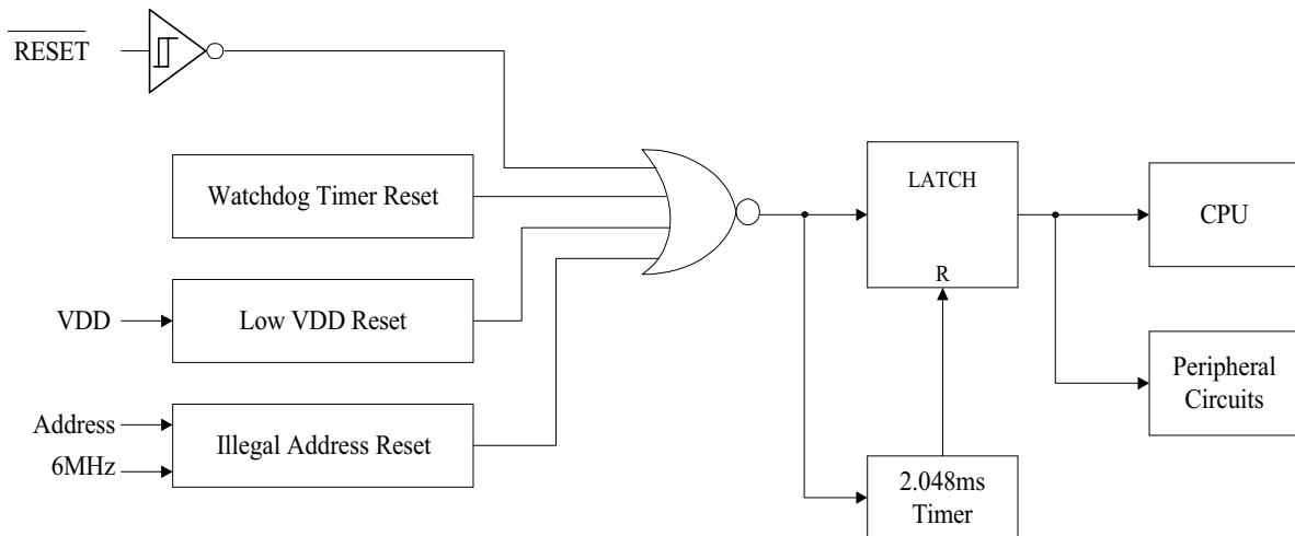
Fig. 1 Reset Signals
