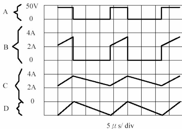
Switching Waveforms
