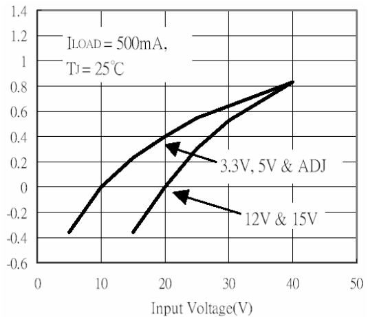
Line Regulator
