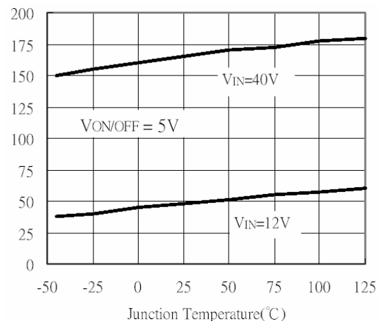
Standby Quiescent Current
