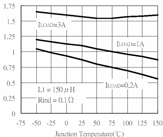
Dropout Voltage
