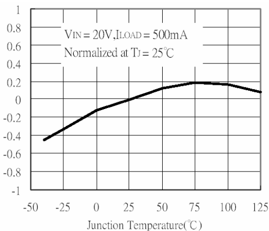
Normalized Output Voltage
