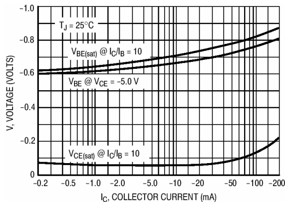
Fig 3. "On" Voltages
