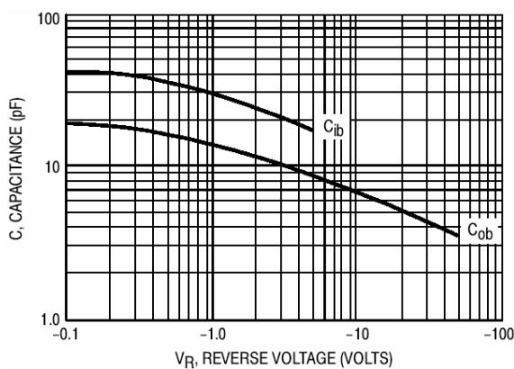
Fig 5. Capacitances
