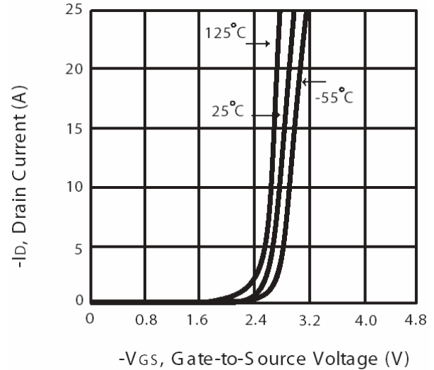
Fig 2. Transfer Characteristics
