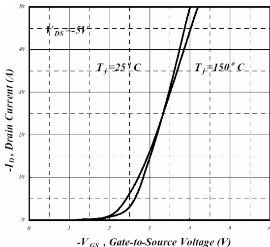
Fig 11. Transfer Characteristics
