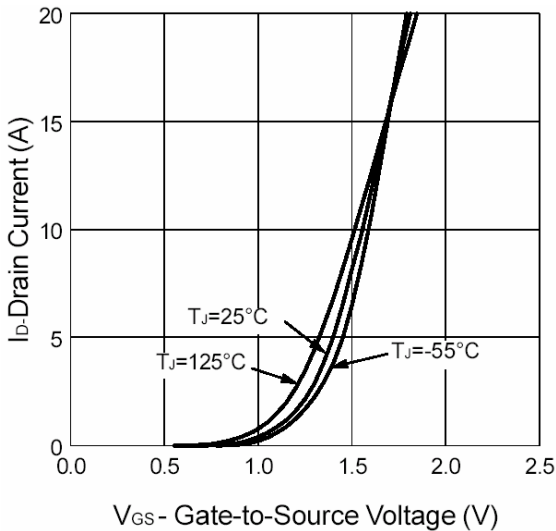
Fig 9. Transfer Characteristics
