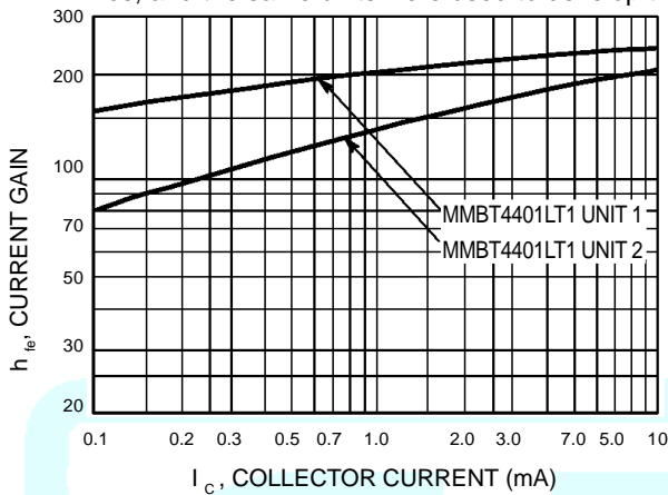
Figure 11. Current Gain
