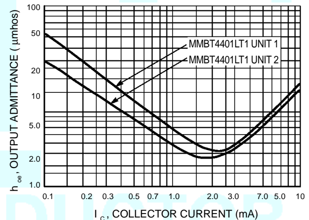
Figure 14. Output Admittance
