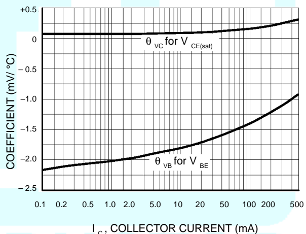
Figure 18. Temperature Coefficients
