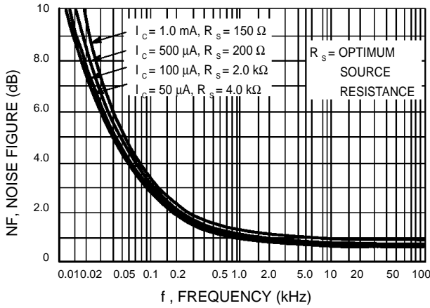
Figure 9. Frequency Effects
