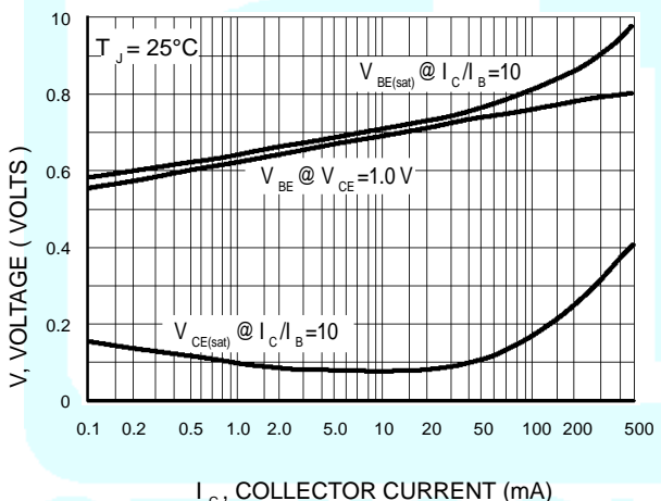
Figure 17. "On" Voltages
