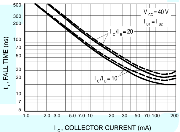
Figure 6. Fall Time
