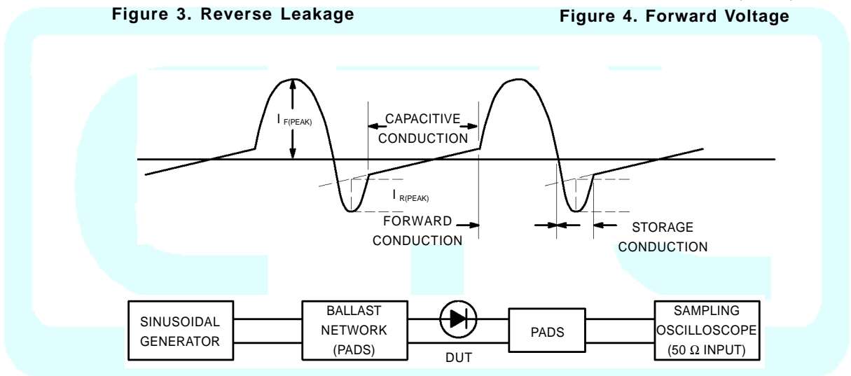
Figure 5. Krakauer Method of Measuring Lifetime
