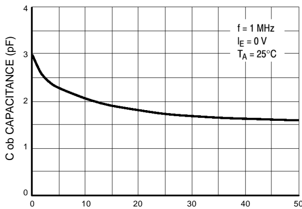
Figure 4. Output Capacitance
