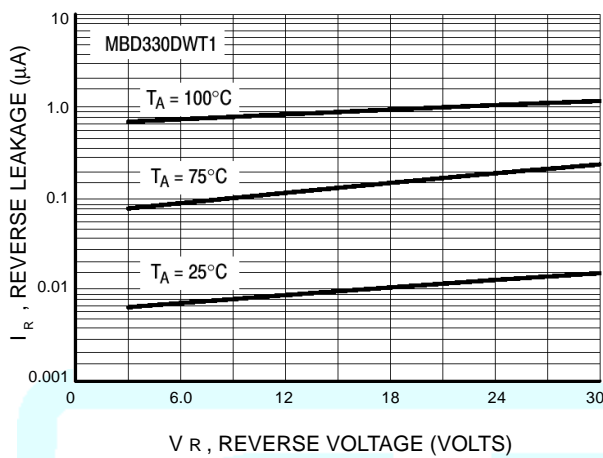
Figure 8. Reverse Leakage
