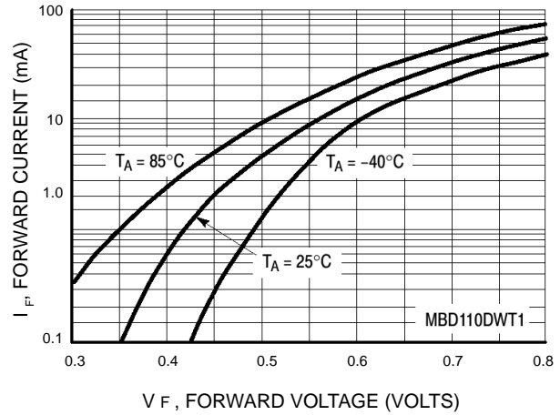
Figure 2. Forward Voltage
